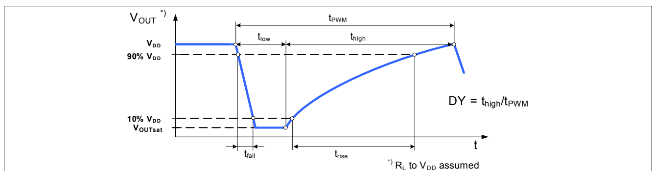
Figure 5-1 Output Characteristic
