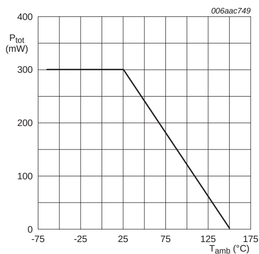
Fig 1. Per device: Power derating curve
