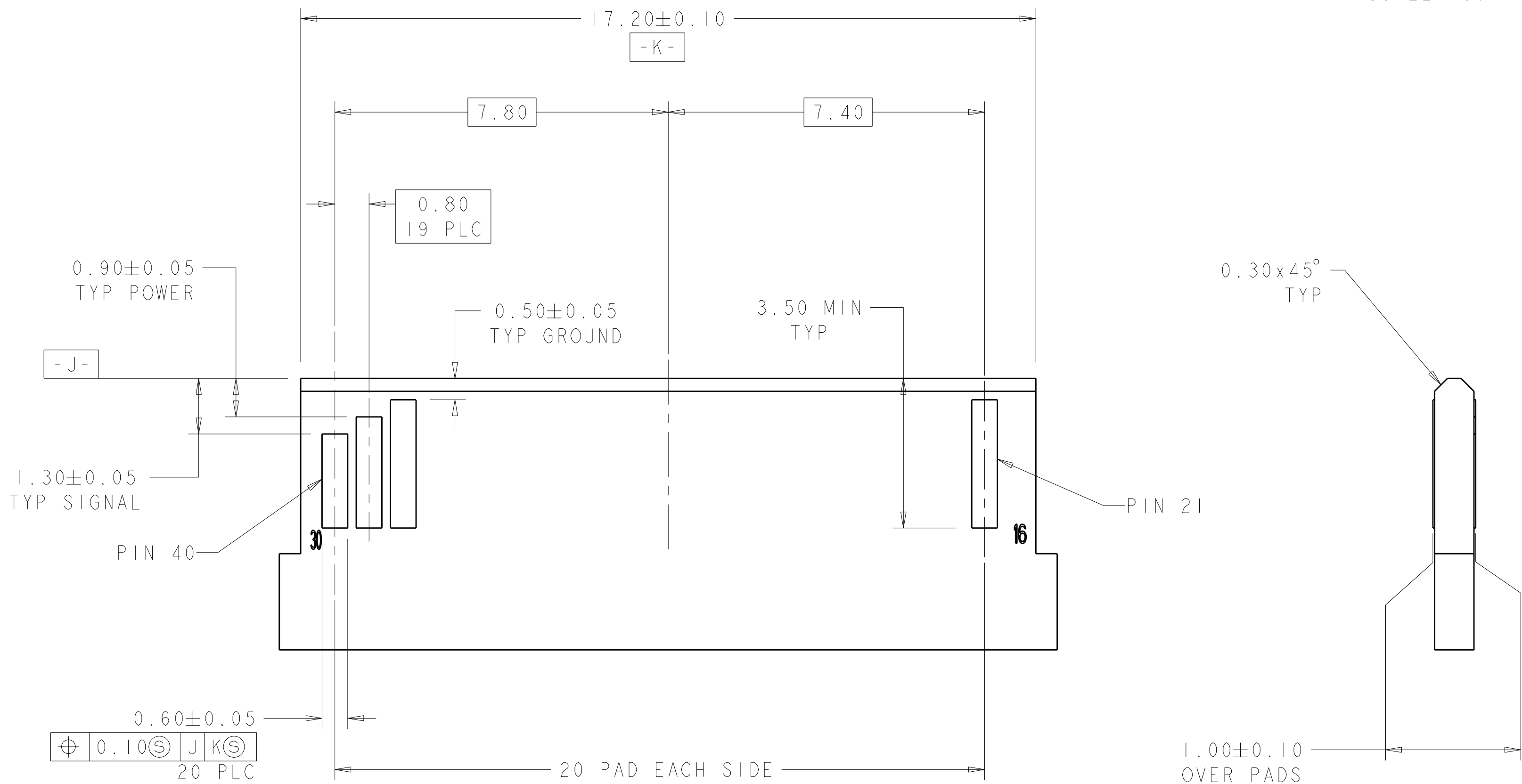
RECOMMENDED PCB LAYOUT DETAIL CONNECTOR MOUNTING SIDE SCALE 8:1
