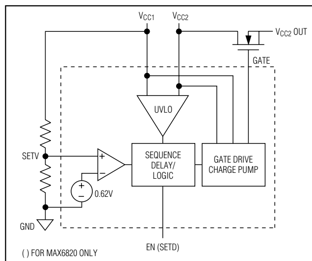
Figure 1. Functional Diagram
