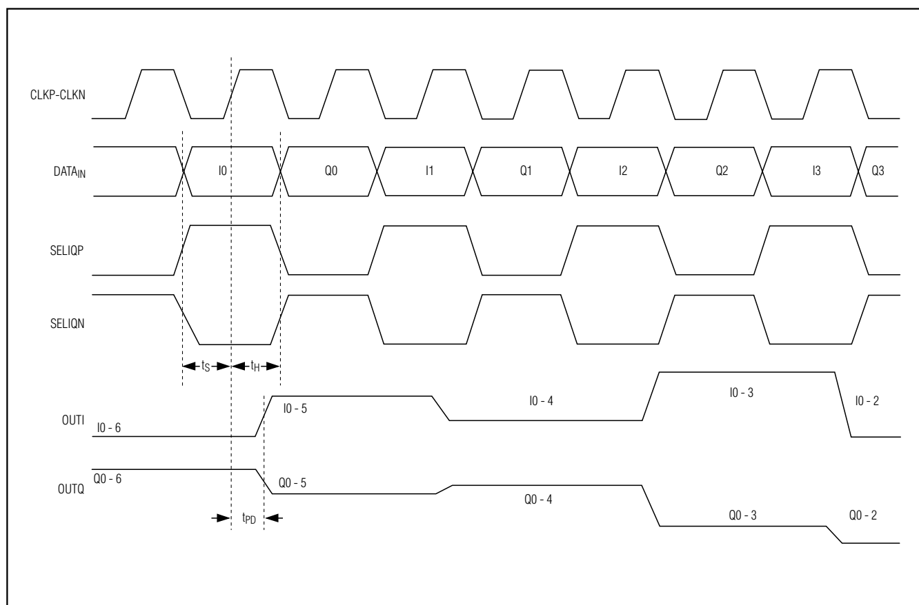
Figure 4. Timing Diagram
