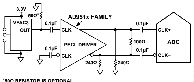
Figure 64. Differential PECL Sample Clock
