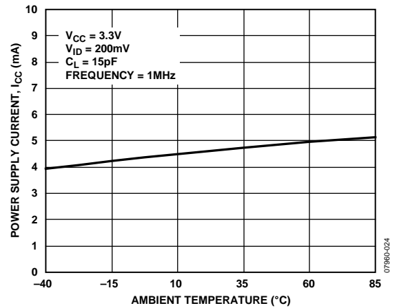
Figure 10. Power Supply Current vs. Ambient Temperature
