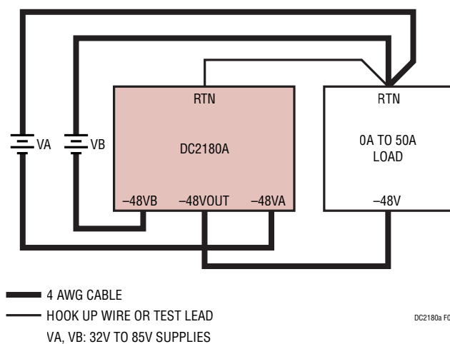
Figure 1. Test Setup
