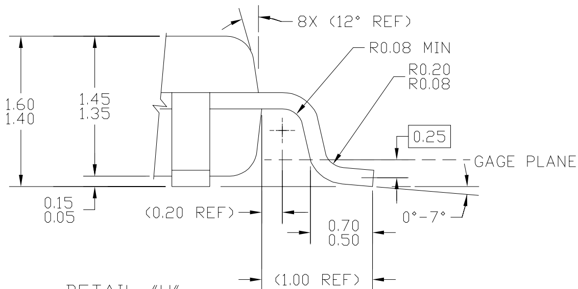
DETAIL "H"
