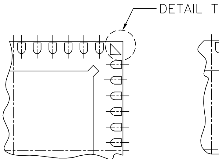
DETAIL M PIN 1 BACKSIDE IDENTIFIER OPTION2
