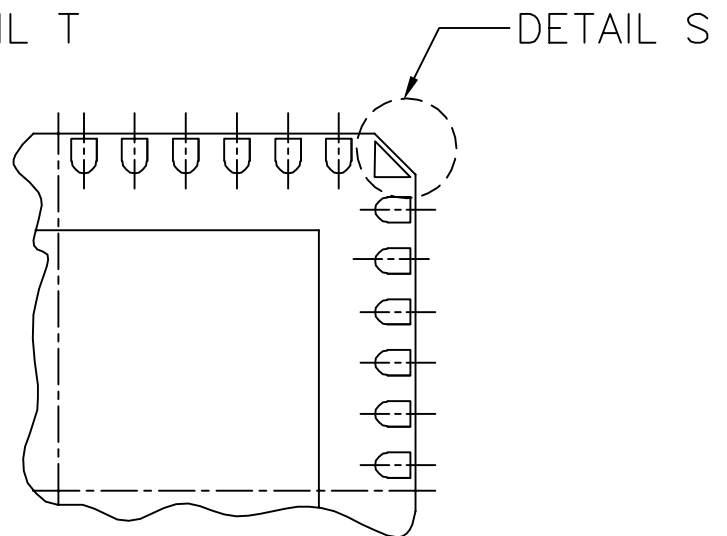
DETAIL M PIN 1 BACKSIDE IDENTIFIER OPTION3
