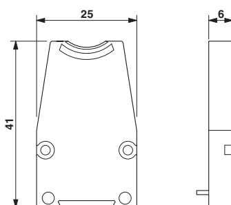
Dimensional drawing
