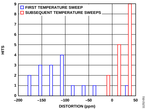
Figure 49. Thermal Hysteresis
