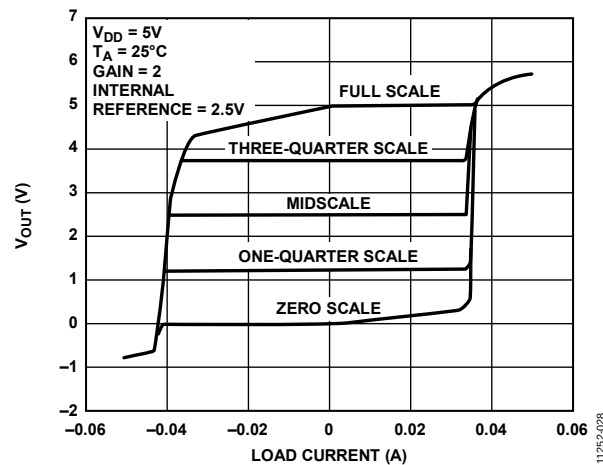
Figure 26. Source and Sink Capability at V_{DD} = 5V
