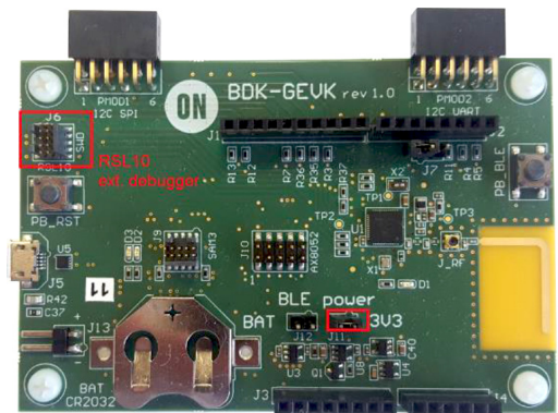
Figure 1. Board Photo
