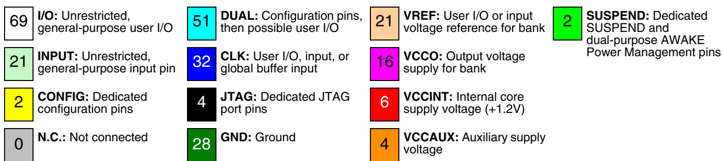
Figure 21: XC3S200A and XC3S400A FT256 Package Footprint (Top View)
