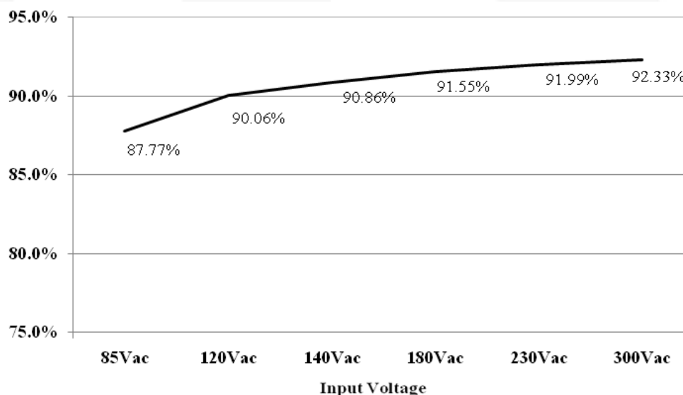
Figure 17. System Efficiency
