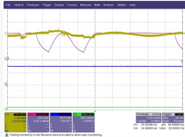
Figure 42. V IN = 300 V AC / 50 Hz, 10% Dim
