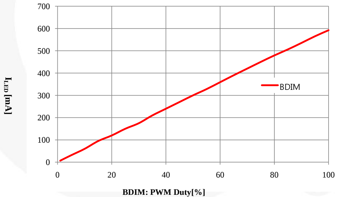
Figure 70. PWM Characteristics
