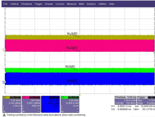
Figure 61. Rated Load [2 ms/div]
