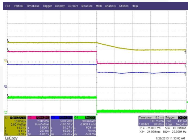
Figure 24. PS-OFF [5 ms/div]
