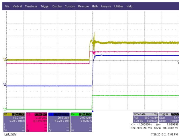
Figure 35. PS-ON
