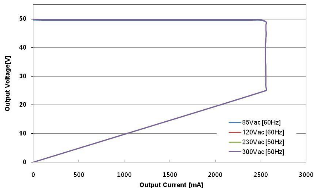
Figure 20. Constant-Current Regulation, Measured by E-Load [CR Mode]
