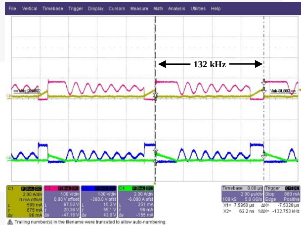
Figure 64. 10% Load [2 us/div]
