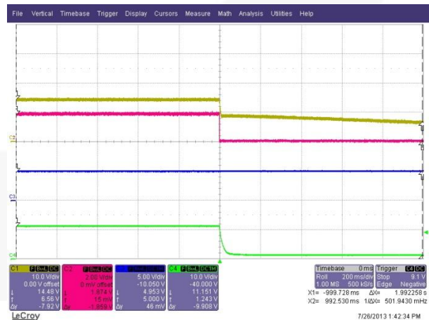
Figure 28. PS-OFF
