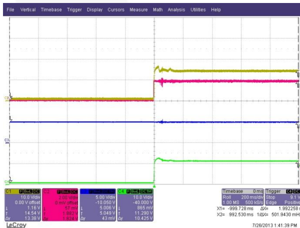
Figure 27. PS-ON
