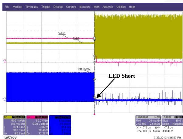
Figure 71. LED Short
