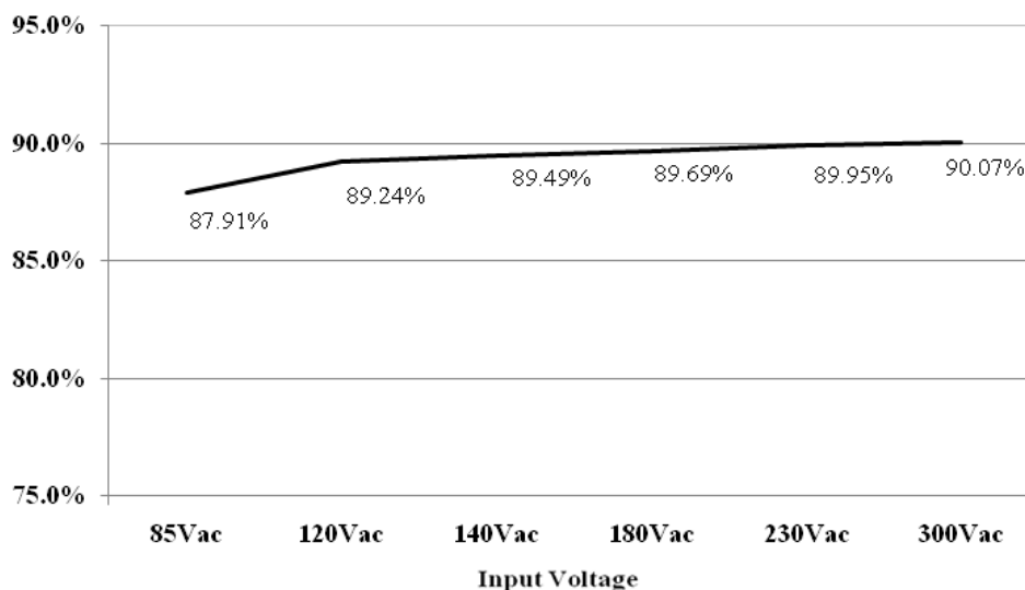
Figure 18. System Efficiency
