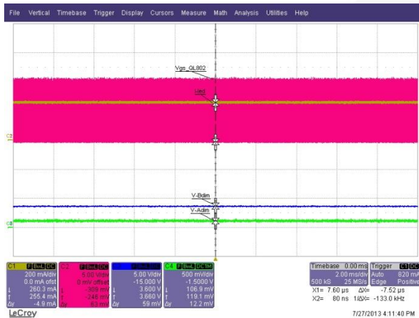
Figure 65. 10% ADIM [2 ms/div]
