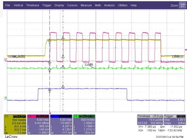
Figure 68. 1% BDIM [10 μs/div]
