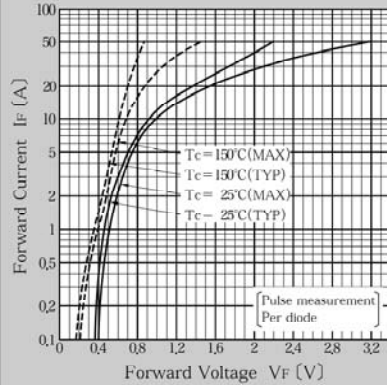
Forward Voltage
