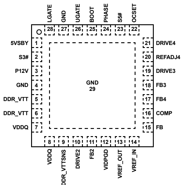
ISL6537 (6x6 QFN) TOP VIEW
