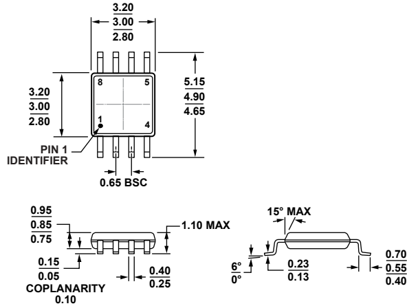
COMPLIANT TO JEDEC STANDARDS MO-187-AA Figure 85. 8-Lead Mini Small Outline Package [MSOP] (RM-8)
