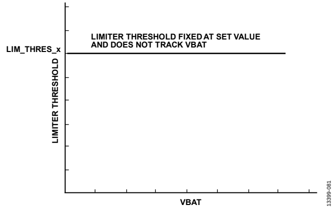
Figure 81. Limiter Fixed (LIM_EN x = 0b11, VBAT_TRACK x = 0b0)
