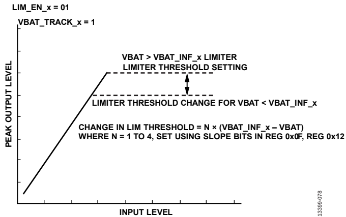
Figure 78. Limiter Fixed (LIM_EN x = 0b01, VBAT_TRACK x = 0b1)
