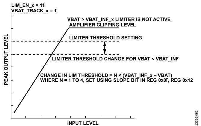
Figure 82. Limiter Example (LIM_EN x = 0b11, VBAT_TRACK x = 0b1)
