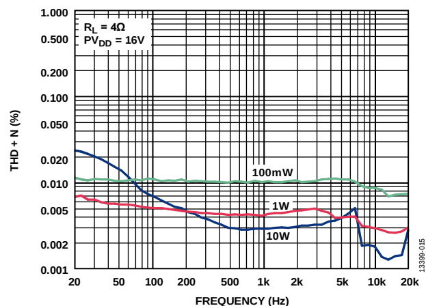
Figure 17. THD + N vs. Frequency, R_L = 4\Omega , P_{VDD} = 16\text{ V}
