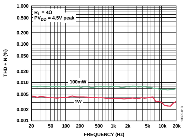
Figure 15. THD + N vs. Frequency, R_L = 4\Omega , P_{VDD} = 4.5\text{ V peak}
