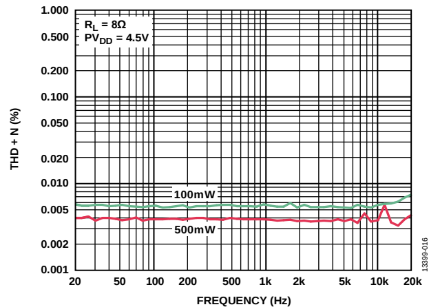
Figure 18. THD + N vs. Frequency, R_L = 8\Omega , P_{VDD} = 4.5\text{ V}
