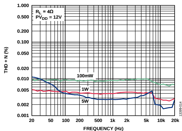
Figure 16. THD + N vs. Frequency, R_L = 4\Omega , P_{VDD} = 12\text{ V}
