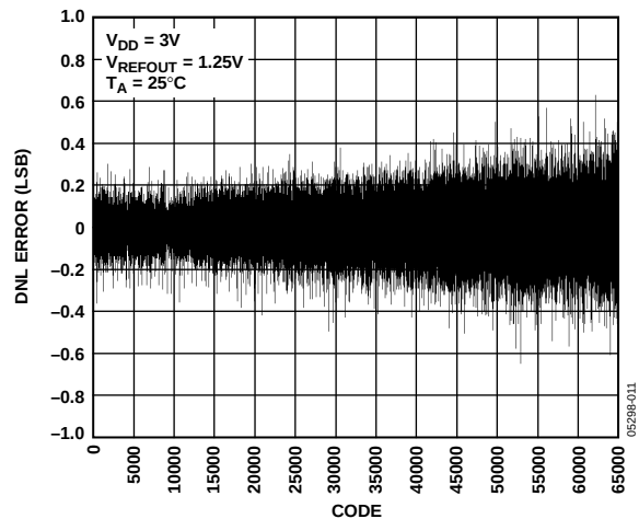
Figure 11. DNL—AD5666-1
