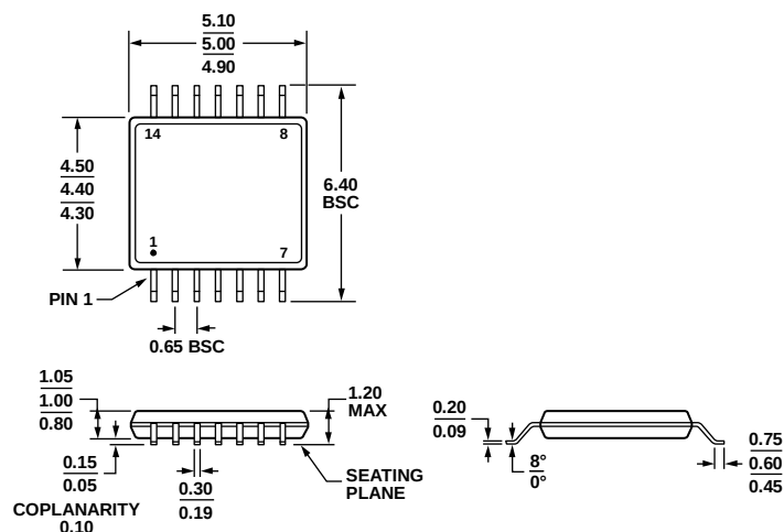
Figure 45. 14-Lead Thin Shrink Small Outline Package [TSSOP] (RU-14) Dimensions shown in millimeters
