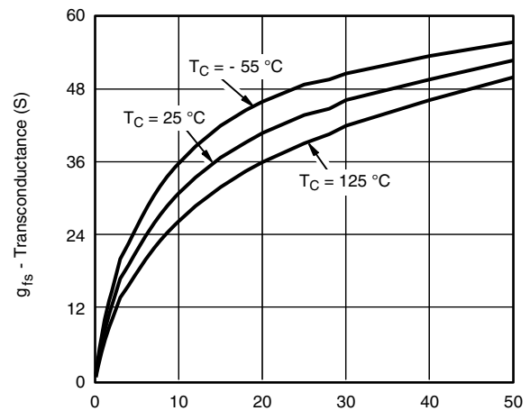
Transconductance
