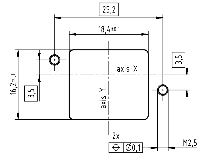
panel cutting
