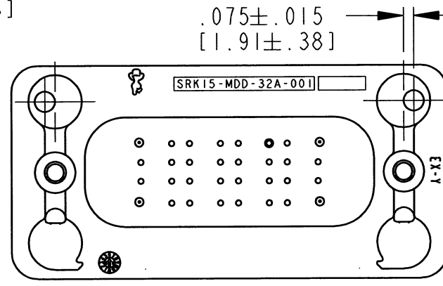
KEY ARRANGEMENT -D- SRK15-MDD-32A-001
