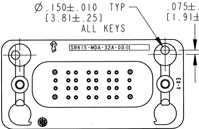
KEY ARRANGEMENT -A- SRK15-MDA-32A-001
