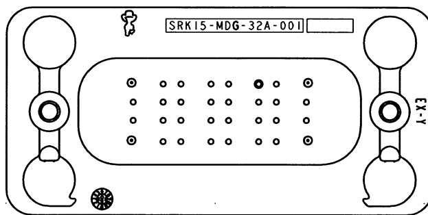
KEY ARRANGEMENT -G- SRK15-MDG-32A-001
