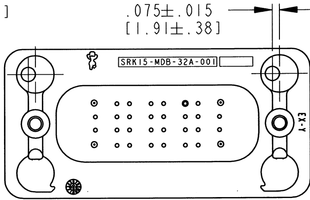
KEY ARRANGEMENT -B- SRK15-MDB-32A-001
