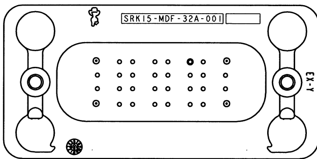
KEY ARRANGEMENT -F- SRK15-MDF-32A-001
