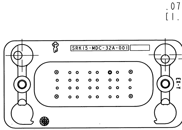
KEY ARRANGEMENT C- SRK15-MDC-32A-001
