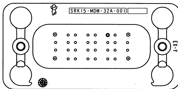
KEY ARRANGEMENT -H- SRK15-MDH-32A-001
