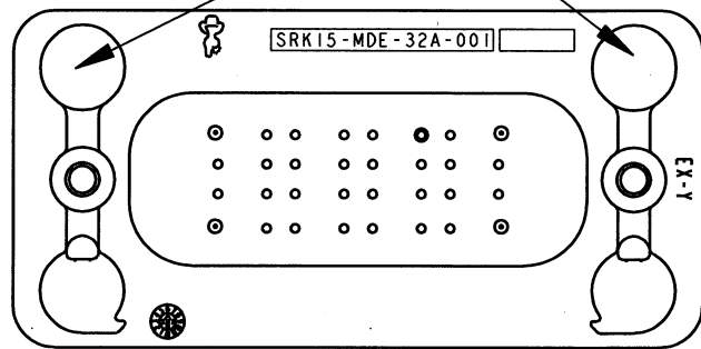
KEY ARRANGEMENT -E- SRK15-MDE-32A-001
