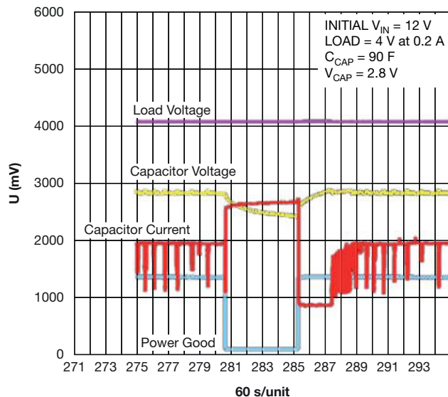
Fig. 1A - 196HVC 90 F - 2.8 V Backup Time &gt; 10 minutes
