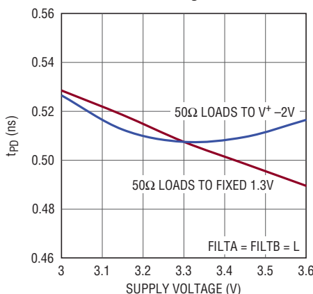
t_{PD} vs Supply Voltage and Termination Voltage
