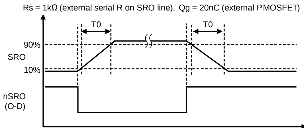
Figure 2. SRO Soft Turn ON and OFF Timing
