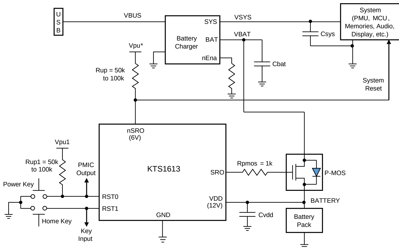
Figure 4. Application Circuit
