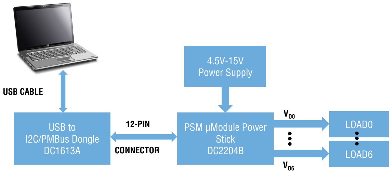
Figure 2. DC2204B Test Setup
