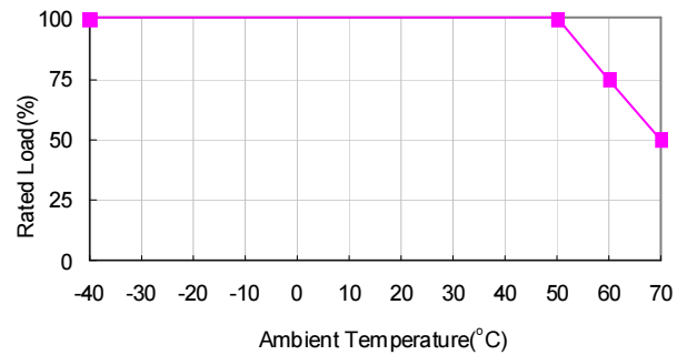
Derating curve:
