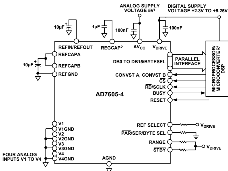
Figure 37. Typical Connection Diagram
