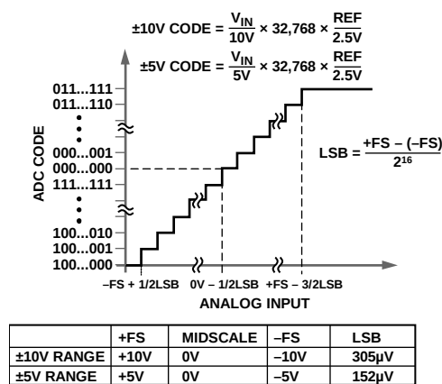
Figure 33. Transfer Characteristics
