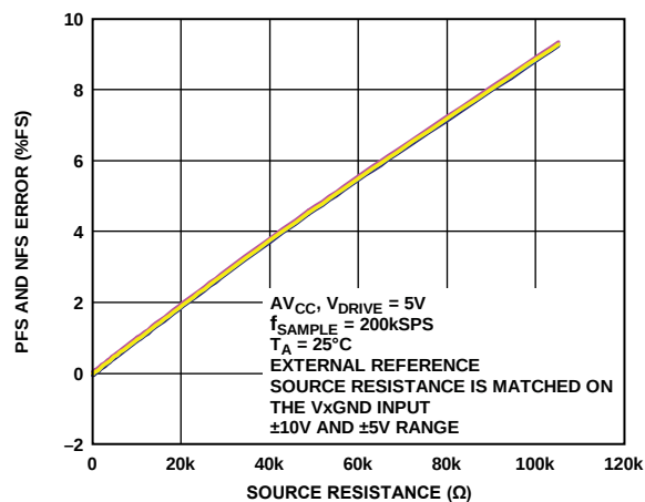
Figure 18. PFS and NFS Error vs. Source Resistance
