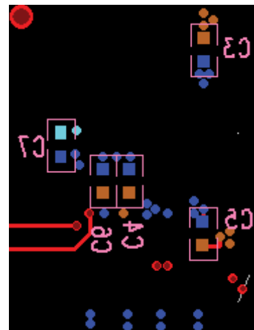
Figure 42. Bottom Layer Decoupling
