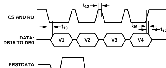
Figure 5. \overline{\text{CS}} and \overline{\text{RD}} , Linked Parallel Mode
