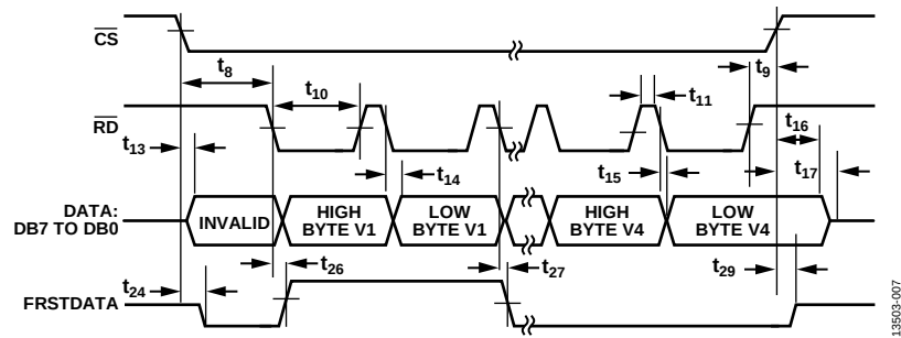
Figure 7. Parallel Byte Mode Read Operation
