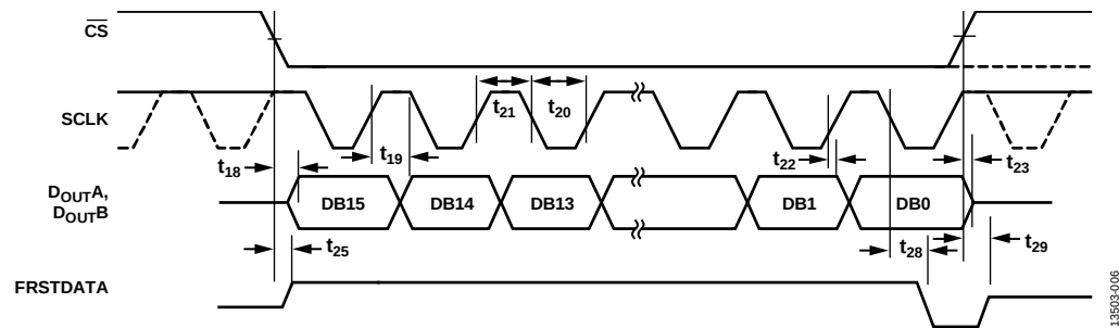
Figure 6. Serial Read Operation
