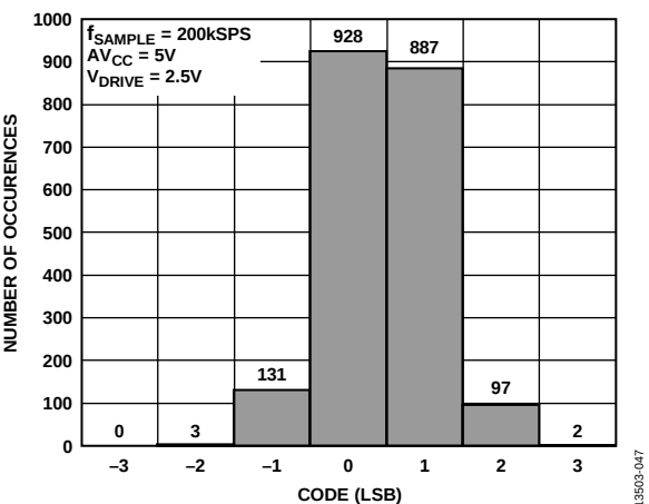
Figure 27. Histogram of Codes (Six Codes)
