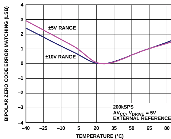
Figure 20. Bipolar Zero Code Error Matching Between Channels
