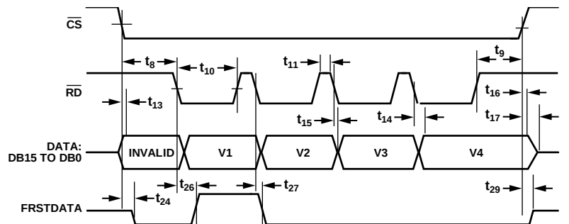
Figure 4. Parallel Mode, Separate \overline{\text{CS}} and \overline{\text{RD}} Pulses
