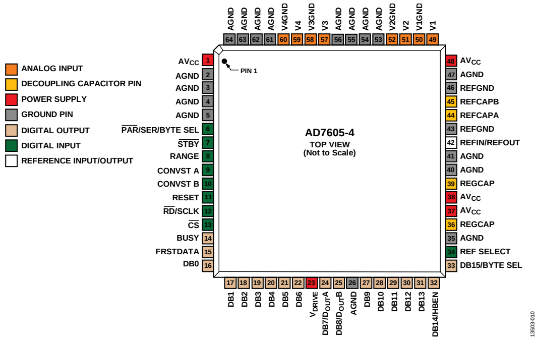
Figure 8. Pin Configuration
