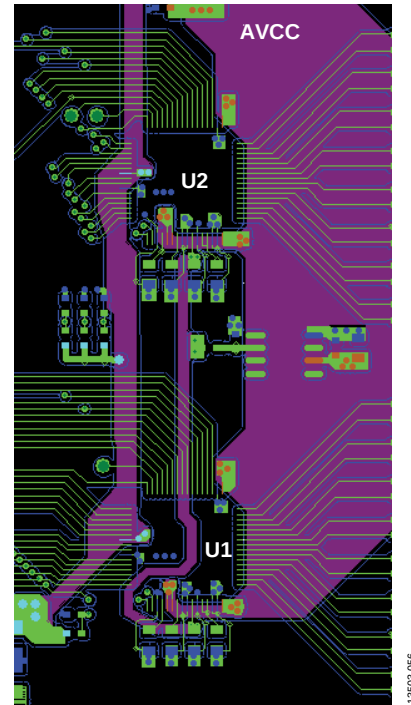
Figure 43. Layout for Multiple AD7605-4 Devices—Top Layer and Supply Plane Layer
