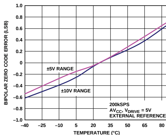
Figure 19. Bipolar Zero Code Error vs. Temperature
