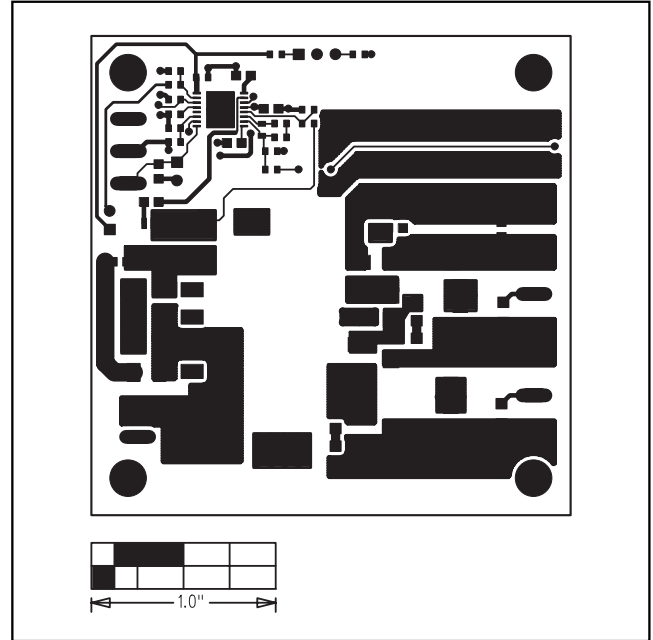
Figure 3. MAX15005A EV Kit PCB Layout—Component Side
