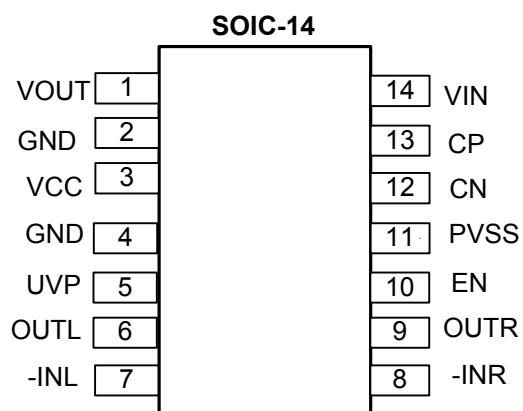
Figure 1 Pin Assignment
