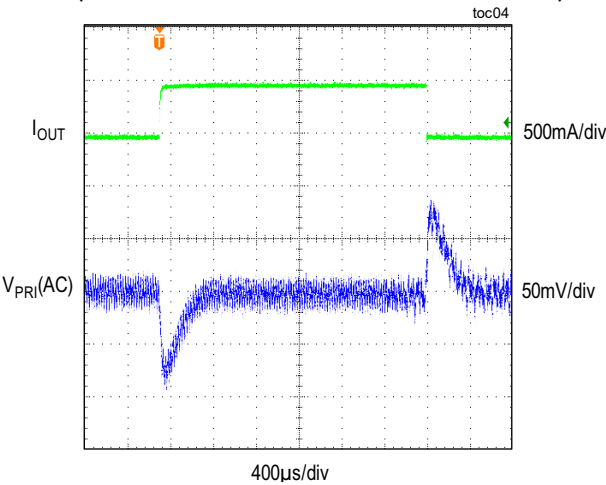
PRIMARY LOAD TRANSIENT RESPONSE (LOAD CURRENT STEPPED FROM 500mA TO 1A)
