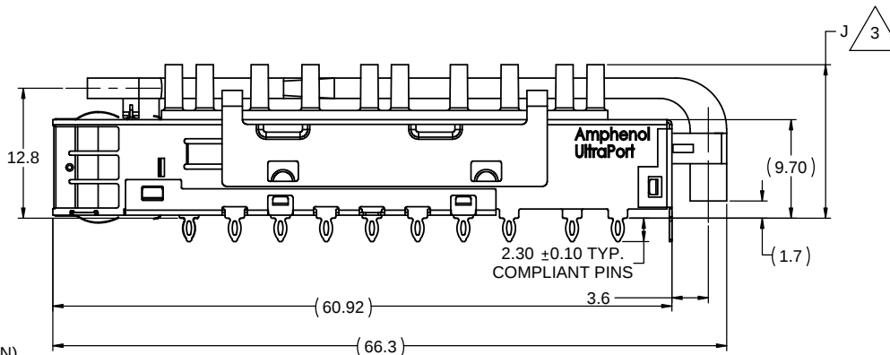
VIEW WITH DUAL BARREL LIGHT PIPE AND ROUND PIN HEAT SINK (NO DUST COVER) (P/N U95-T151-101A)
