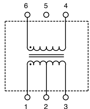
Schematic D
