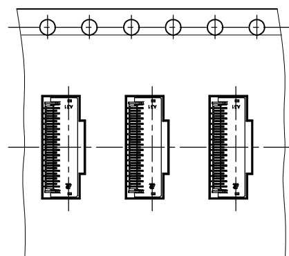
VIEW W
