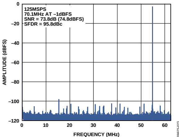
Figure 11. Single-Tone FFT with f_{IN} = 70.1 MHz
