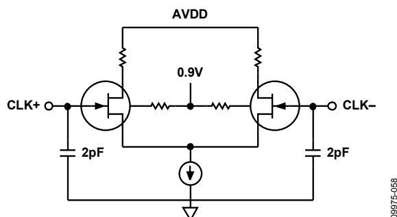
Figure 51. Equivalent Clock Input Circuit
