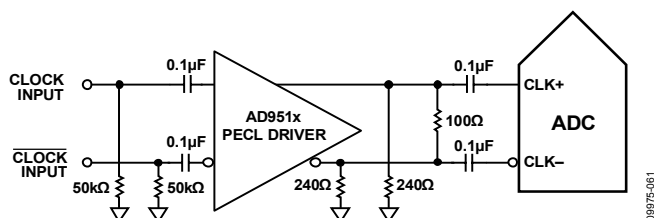
Figure 54. Differential PECL Sample Clock (Up to 1 GHz)
