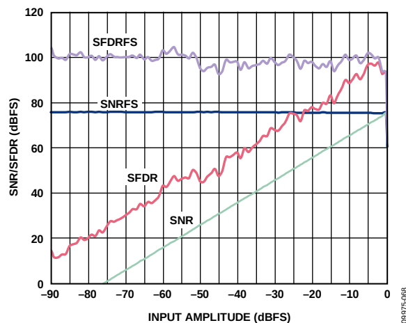
Figure 16. SNR/SFDR vs. Input Amplitude (AIN) with f_{IN} = 9.7 MHz
