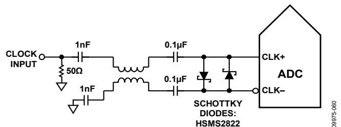
Figure 53. Balun-Coupled Differential Clock (Up to 1 GHz)
