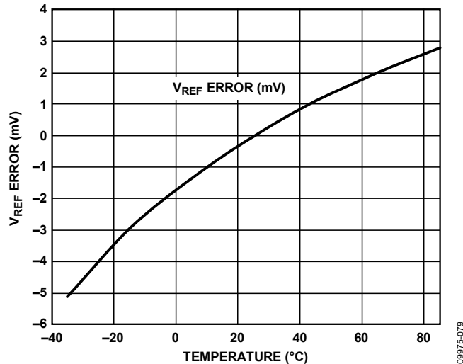
Figure 50. Typical V_{REF} Drift
