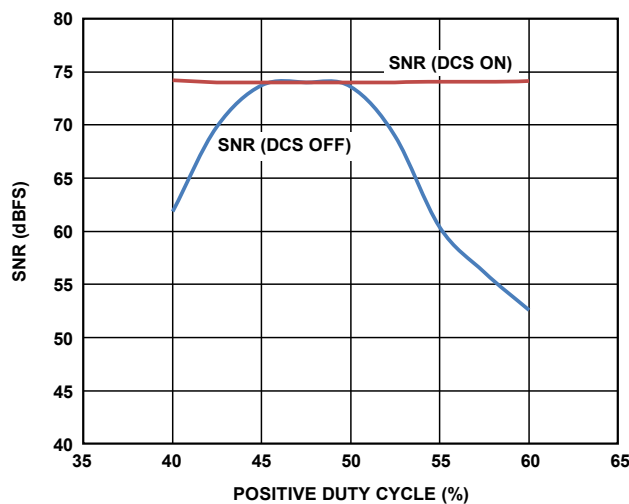
Figure 57. SNR vs. DCS On/Off
