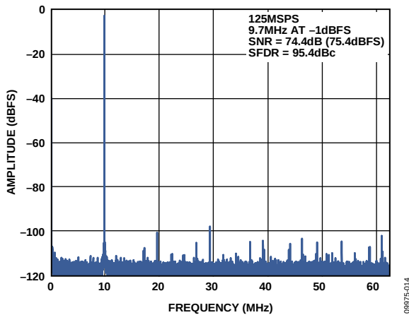
Figure 9. Single-Tone FFT with f_{IN} = 9.7 MHz
