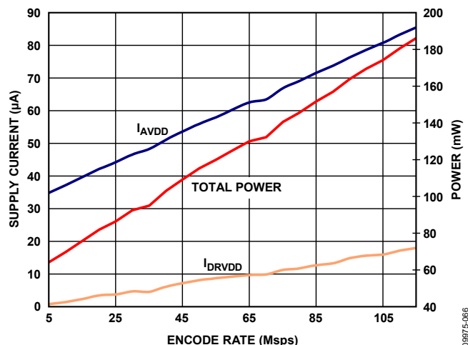
Figure 60. AD9648-105 Power and Current vs. Clock Rate (1.8 V CMOS Output Mode)
