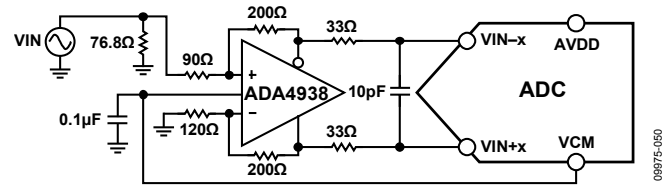
Figure 44. Differential Input Configuration Using the ADA4938-2
