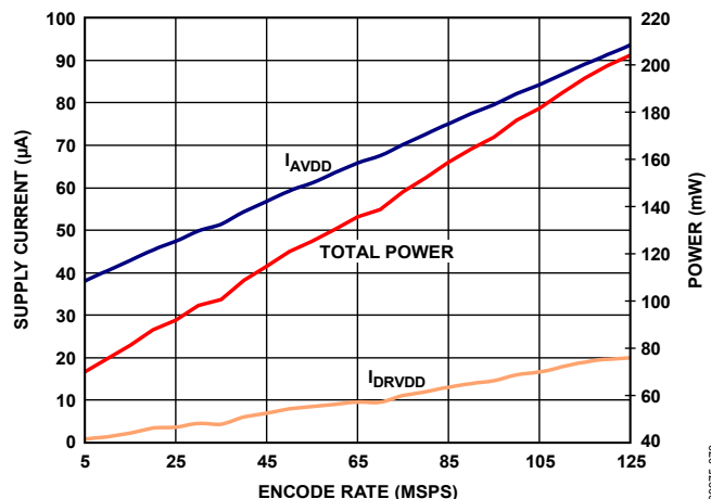
Figure 59. AD9648-125 Power and Current vs. Clock Rate (1.8 V CMOS Output Mode)
