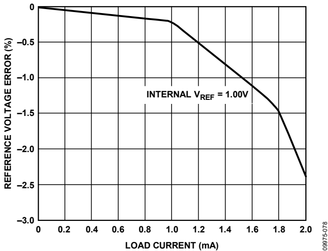
Figure 49. VREF Accuracy vs. Load Current
