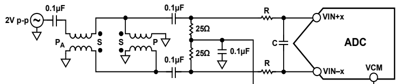
Figure 46. Differential Double Balun Input Configuration
