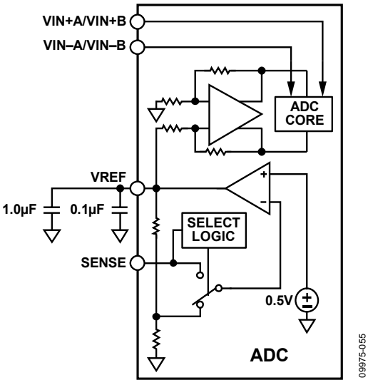
Figure 48. Internal Reference Configuration
