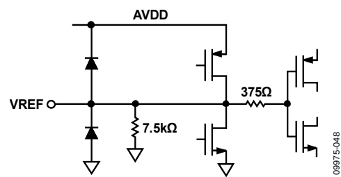
Figure 41. Equivalent VREF Circuit
