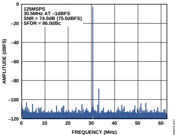
Figure 10. Single-Tone FFT with f_{IN} = 30.5 MHz
