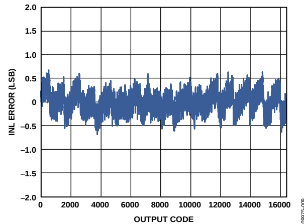
Figure 33. INL Error with f_{IN} = 9.7 MHz
