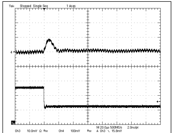
Fig-2.5V-7: Output voltage response for V_{out}=2.5V to negative load current step change from 5A to 2.5A with slew rate of -5A/\mu s at V_{in}=12V . C_o=47\mu F \times 2 ceramic.
