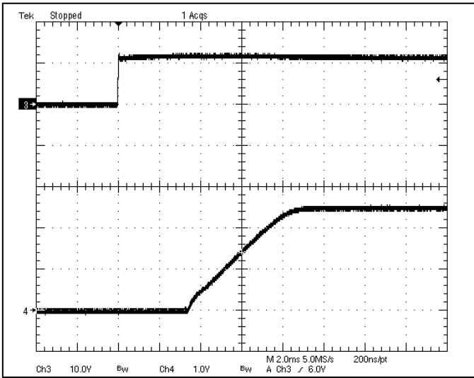
Fig-2.5V-4: Turn-on transient for V_{out}=2.5V with application of V_{in} at full rated load current (resistive) and 47\mu F \times 2 external capacitance at V_{in}=12V .
