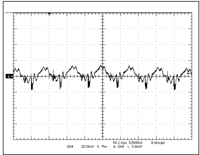
Fig-2.5V-5: Output voltage ripple (20mV/div.) for V_{out}=2.5V at full rated load current into a resistive load with external capacitance 47\mu F \times 2 ceramic + 1\mu F ceramic at V_{in}=12V .
