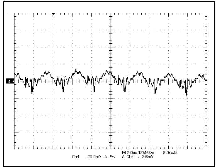
Fig-2.0V-5: Output voltage ripple (20mV/div.) for V_{out}=2.0V at full rated load current into a resistive load with external capacitance 47\mu F \times 2 ceramic + 1\mu F ceramic at V_{in}=12V .
