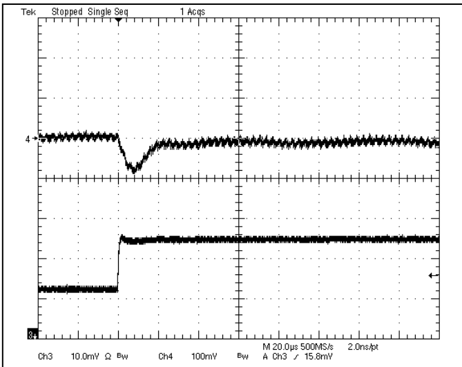
Fig-2.0V-6: Output voltage response for V_{out}=2.0V to positive load current step change from 2.5A to 5A with slew rate of 5A/\mu s at V_{in}=12V . C_o=47\mu F \times 2 ceramic.
