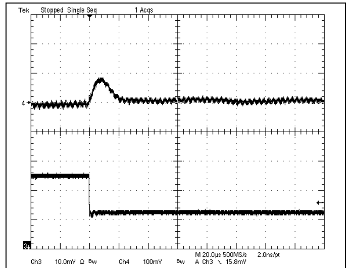
Fig-2.0V-7: Output voltage response for V_{out}=2.0V to negative load current step change from 5A to 2.5A with slew rate of -5A/\mu s at V_{in}=12V . C_o=47\mu F \times 2 ceramic.
