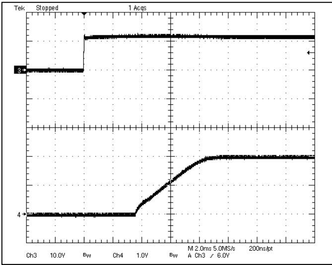
Fig-2.0V-4: Turn-on transient for V_{out}=2.0V with application of V_{in} at full rated load current (resistive) and 47\mu F \times 2 external capacitance at V_{in}=12V .
