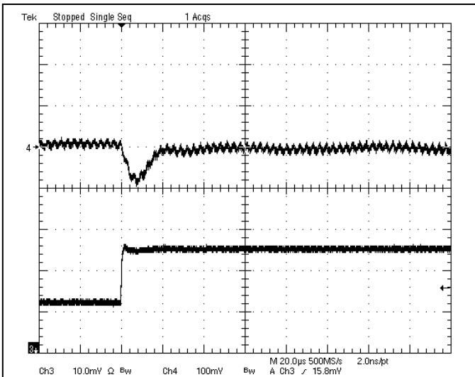
Fig-2.5V-6: Output voltage response for V_{out}=2.5V to positive load current step change from 2.5A to 5A with slew rate of 5A/\mu s at V_{in}=12V . C_o=47\mu F \times 2 ceramic.
