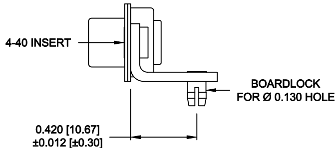
MOUNTING HARDWARE
