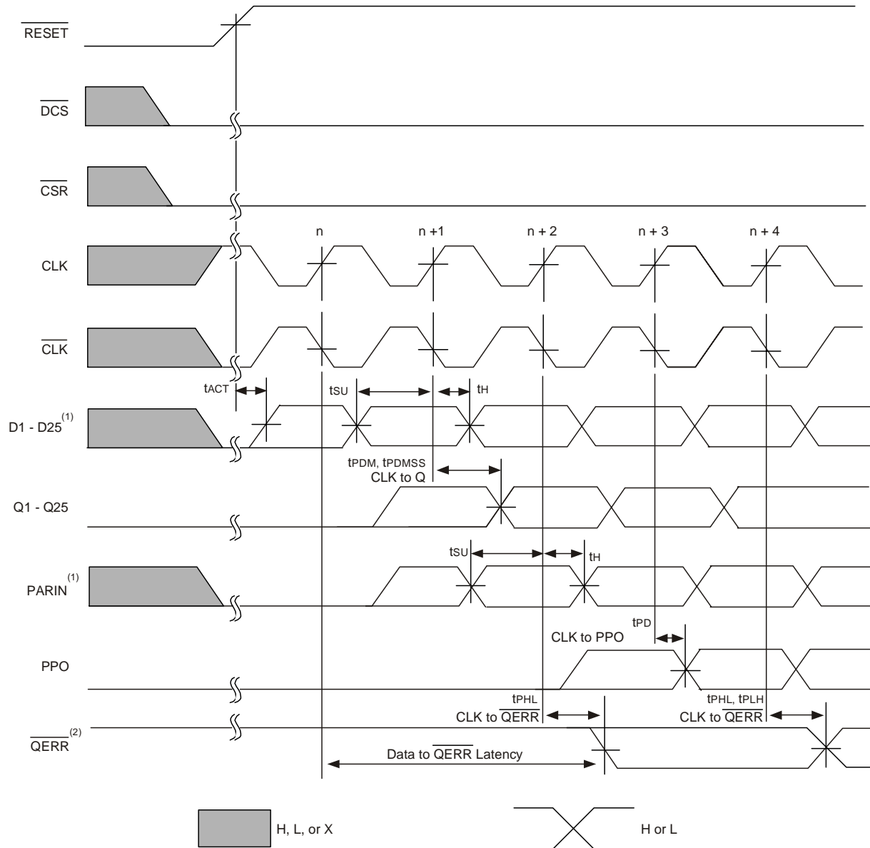
Timing Diagram for SSTUBF32866B Used as a Single Device; C0 = 0, C1 = 0, \overline{RESET} Switches from L to H
