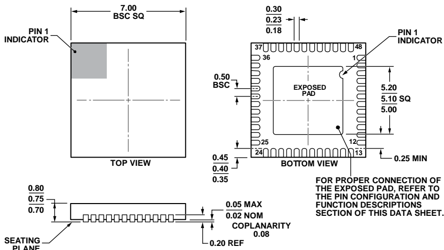
Figure 48. 48-Lead Lead Frame Chip Scale Package [LFCSFP] 7 mm × 7 mm Body and 0.75 mm Package Height (CP-48-4)
