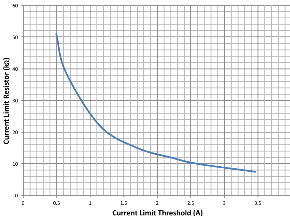
Figure 28. Current Limit Threshold ( I_{\text{os}} ) vs Current Limit Resistor (RLIM)
