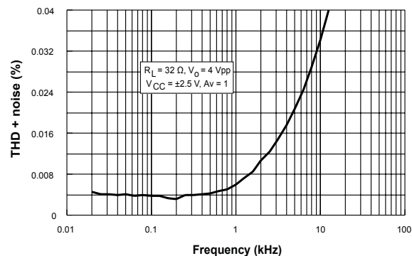
Figure 8. THD + noise vs. frequency ( R_L = 32\text{ }\Omega , V_O = 4\text{ Vpp} , V_{CC} = \pm 2.5\text{ V} , A_v = 1 )
