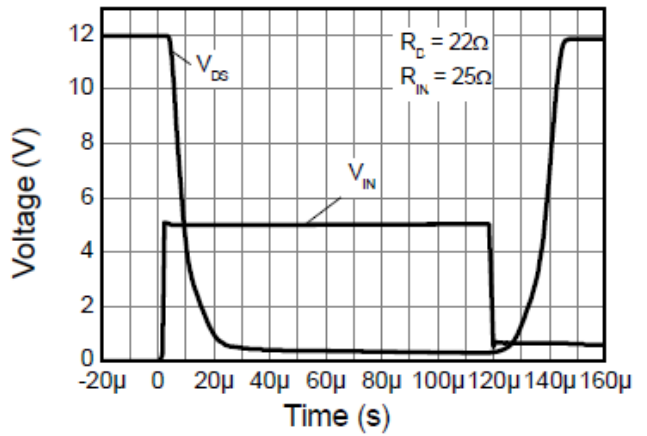
Switching Speed
