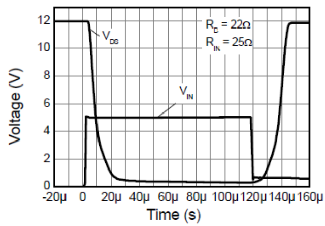
Switching Speed
