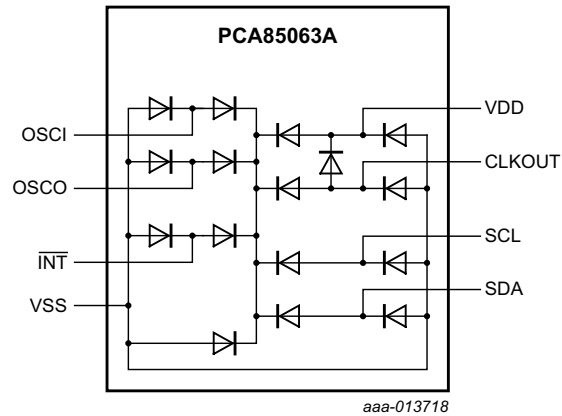
Fig 22. Device diode protection diagram of PCA85063A
