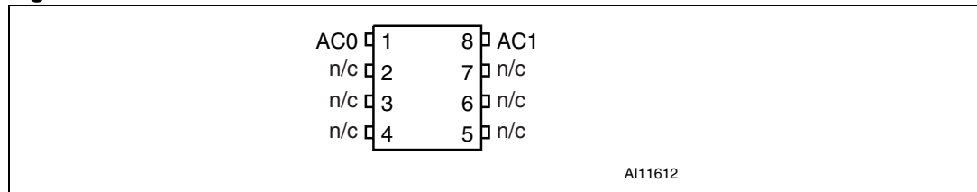
Figure 2. UDFPN8 connections
