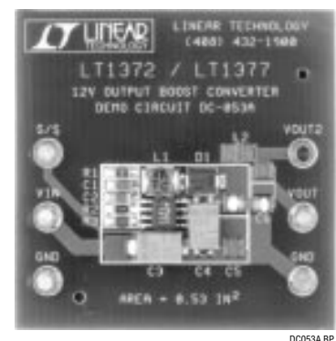
Component Side
