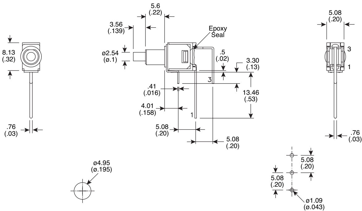
PANEL MOUNTING
