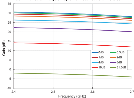
Gain versus Frequency and Attenuation State
