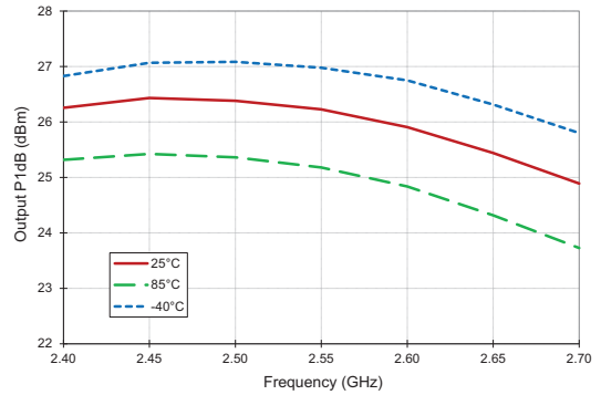
Output P1dB versus Frequency and Temperature
